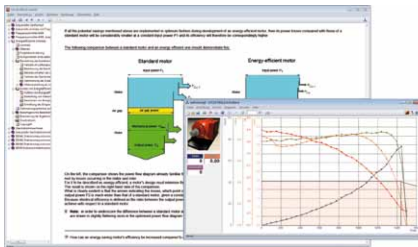
Comparison between standard and energy-efficient motors with the help of characteristic recording in the ILA course titled "Energy-efficient drives".
