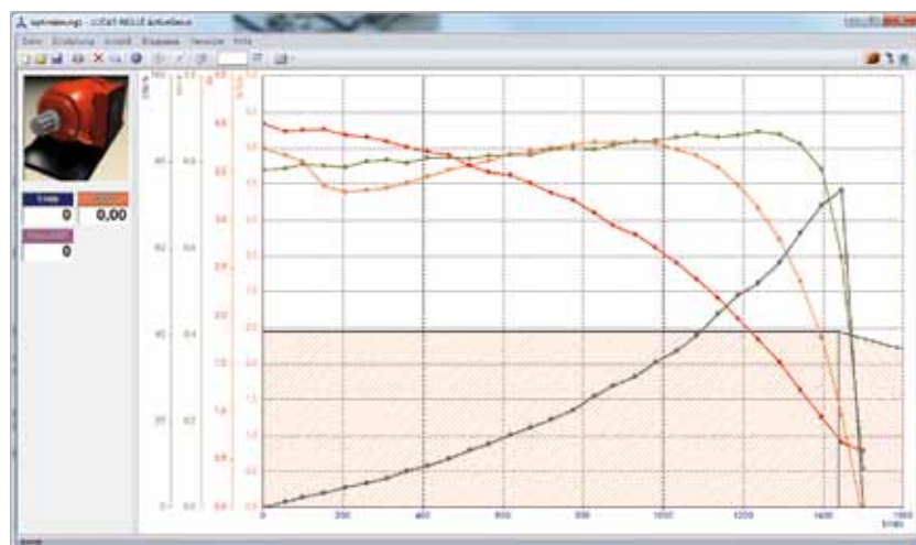
Automatic recording of characteristics by ActiveServo software
